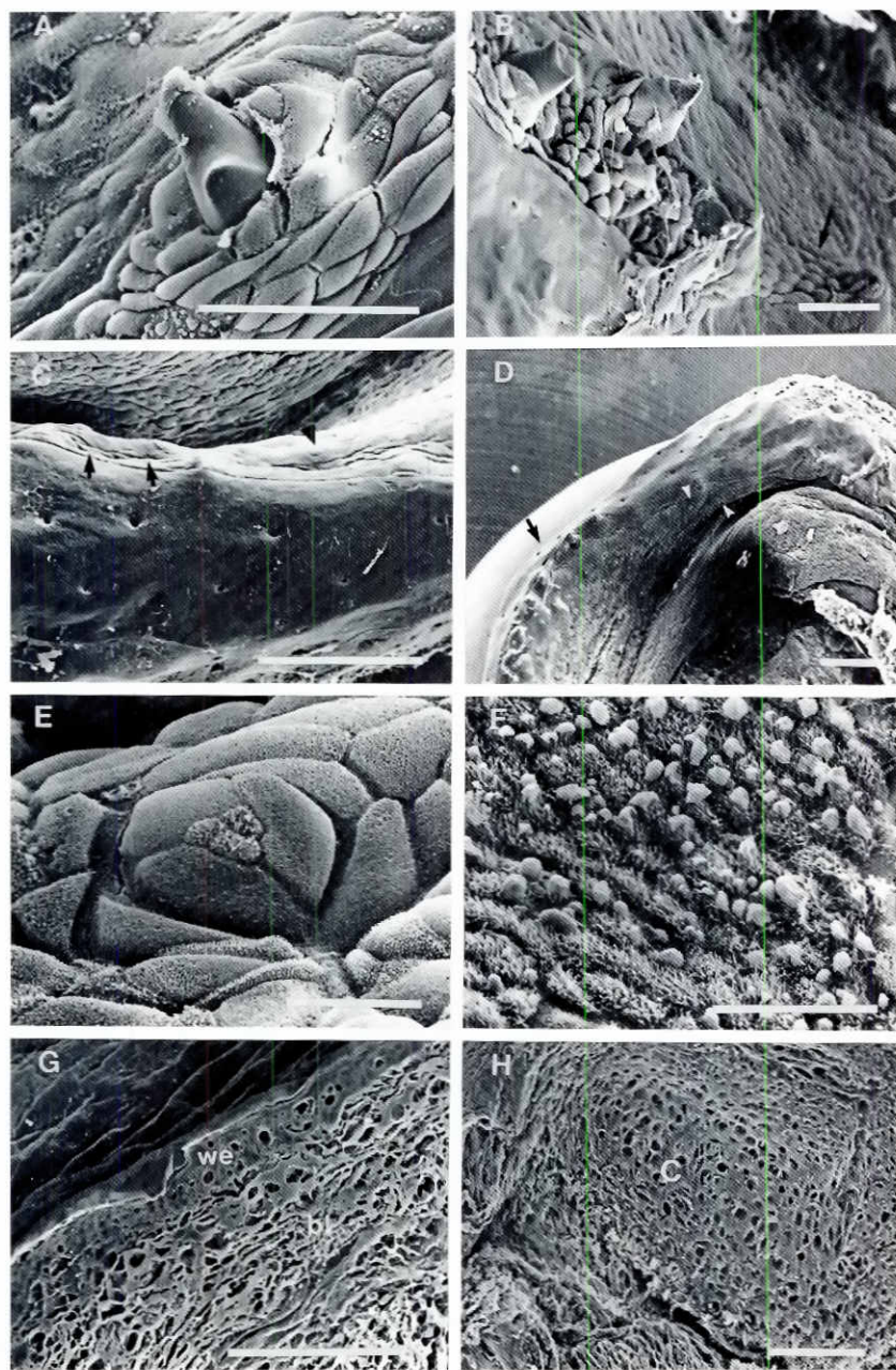
Fig. 4. SEM photographs of regenerating upper and lower jaws. (A) Regenerated bicuspid tooth in a 10 week upper jaw regenerate; scale bar, 50 \mu m. (B) Regenerated teeth and growing dental lamina (arrow) in a 10 week upper jaw regenerate. Scale bar, 50 \mu m. (C) Growing dental lamina (arrows) and regenerated glands (arrowhead) in a 8 weeks lower jaw regenerate. Scale bar, 200 \mu m. (D) Lower magnification photograph of the same jaw as in C; the arrow indicates the level of amputation, and the arrowheads regenerated glands; scale bar, 200 \mu m. (E) Regenerated mucous glands identical to those in the unamputated oral mucosa are found both in 10 week upper (shown here) and lower jaw regenerates; scale bar, 20 \mu m. (F) Sensory ciliated epithelium in a 10 week upper jaw regenerate; scale bar, 50 \mu m. (G) Lower jaw blastema 3 weeks after amputation (view of surface perpendicular to the mandible stump). we: wound epidermis; bl: blastema; scale bar, 200 \mu m. (H) Regenerating cartilage (c) just distal to the level of amputation (view of surface perpendicular to the mandible stump) in a 3 week lower jaw regenerate; scale bar, 200 \mu m.
