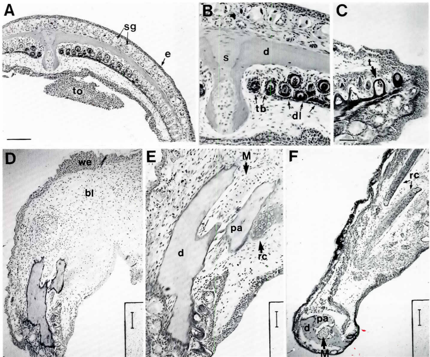
Fig. 3. Haematoxylin and eosin (A-B) and alcian blue-durazol red (C-F) staining of paraffin sections of normal (A-C) and regenerating (D-F) lower jaws. (A) Oblique coronal section. e: epidermis; sg: subepidermal glands; to: tongue. (B) Higher magnification of A: note the tooth buds and the dental lamina; s: median symphysis; d: dentary bone; tb: tooth bud; dl: dental lamina. (C) Sagittal section; the arrow indicates an erupted tooth (t). Coronal section of a 3 week regenerate; a blastema has formed and cartilage condensation is already apparent. bl: blastema; we: wound epithelium. (E) Higher magnification of the regenerating cartilage shown in D. d: dentary bone; M: Meckel's cartilage; pa: prearticular bone; rc: regenerating cartilage. (F) Frontal slightly oblique section of a 4 week regenerate (see E for acronyms). Scale bars, 200 µm.
